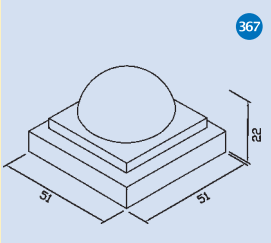
Remata redondo grande
