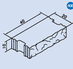
Ladrillo split Alhambra terminal
