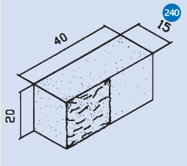
Ladrillo split Alhambra standard
