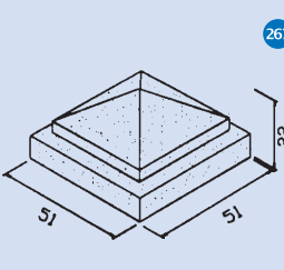
Remate mod. pico
