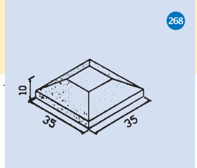
Remate mod. plano
