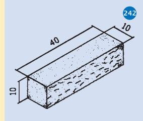
Ladrillo split Alhambra standard
